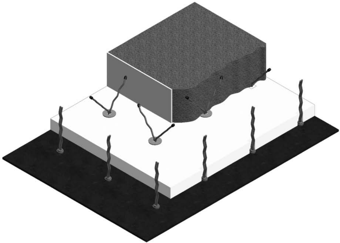
Sample of installation: Product category 1 with rear insulation
